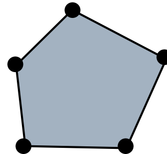
Pentagonal
