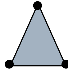
Ternary
